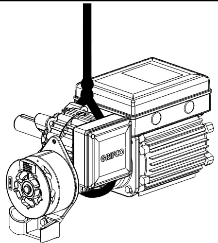
Alignment of door sprocket to output shaft of eDrive +2.0 (see left)
