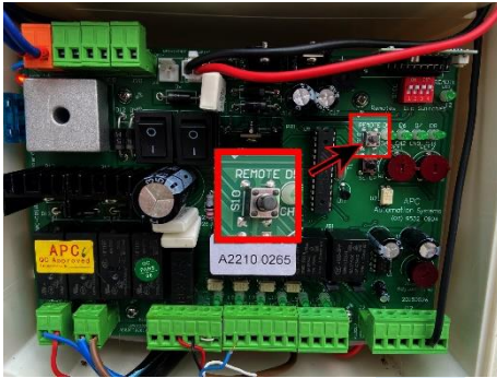
Swing Gate
