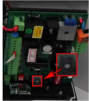
Sliding Gate
